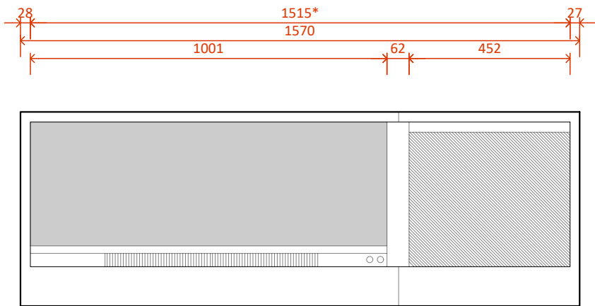
LE1000 MK2 with Single Niche Right - Front
