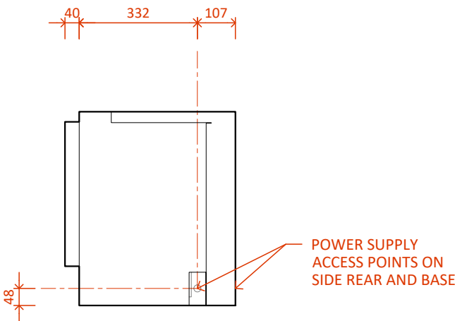
LE1000 MK2 with Single Niche Right - Side
