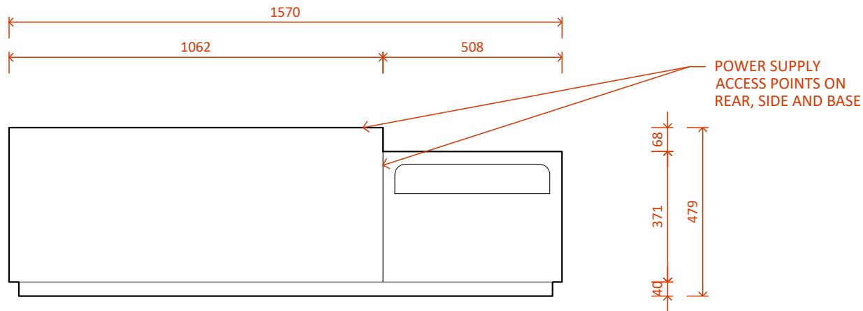
LE1000 MK2 with Single Niche Right - Plan
