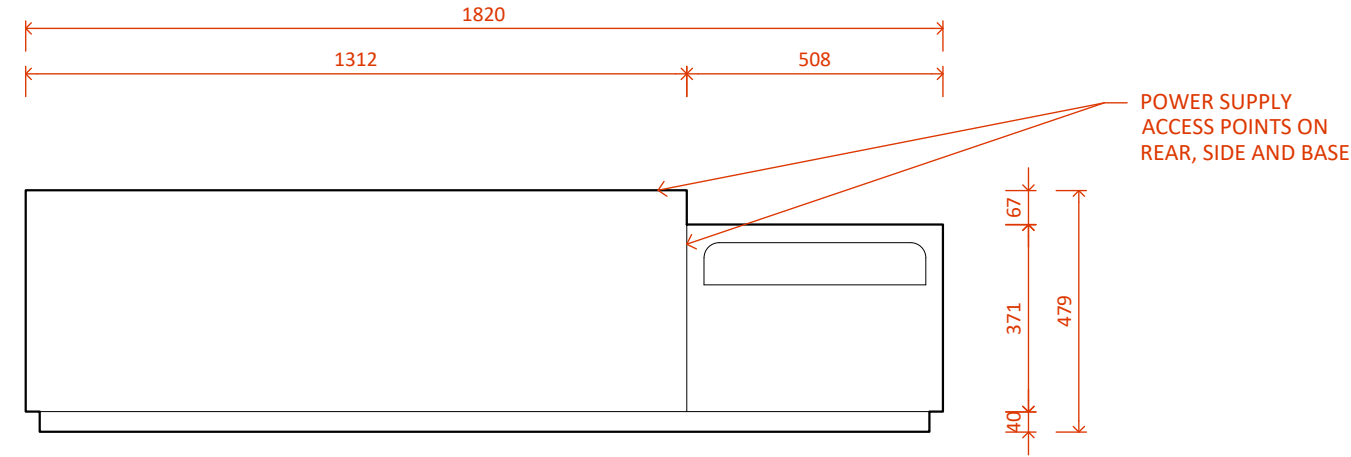
LE1250 MK2 with Single Niche Right - Plan
