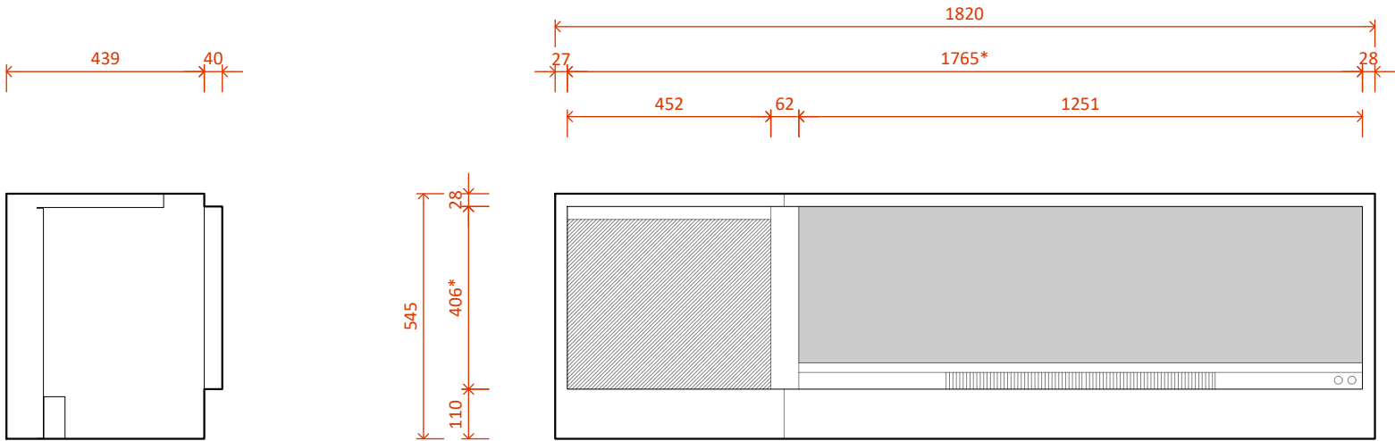
LE1250 MK2 with Single Niche Left - Side
