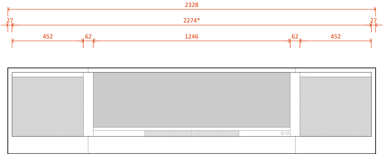
LE1250 MK2 with Double Niche - Front
