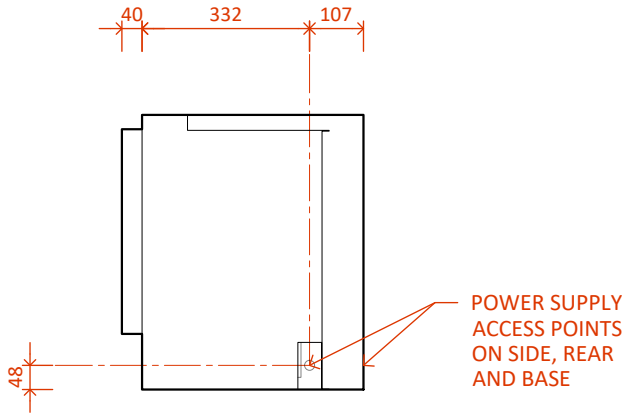
LE1250 MK2 with Single Niche Right - Side
