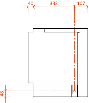
LE1250 MK2 with Double Niche - Side R
