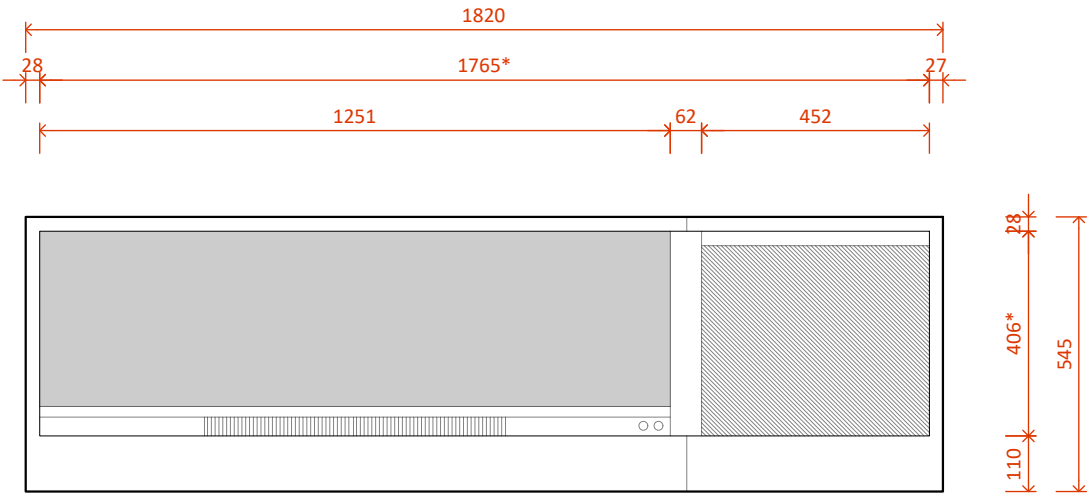
LE1250 MK2 with Single Niche Right - Front
