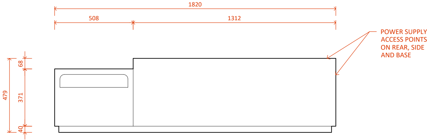
LE1250 MK2 with Single Niche Left - Plan
