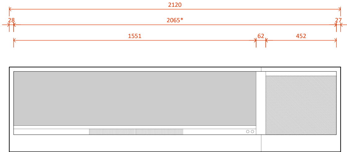
LE1550 MK2 with Single Niche Right - Front
