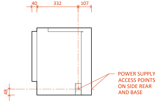
LE1550 MK2 with Single Niche Right - Side
